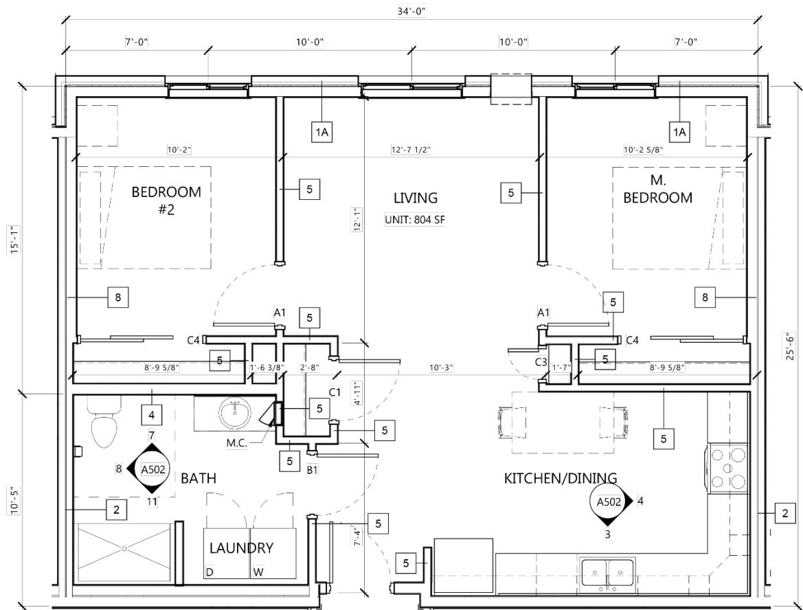
1 UNIT 2 A502 1/4" = 1'-0"
