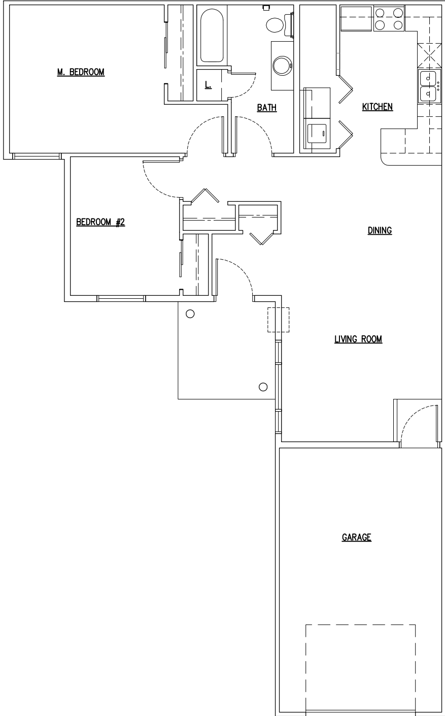
○ UNIT PLAN 'A' (W/ GARAGE)
